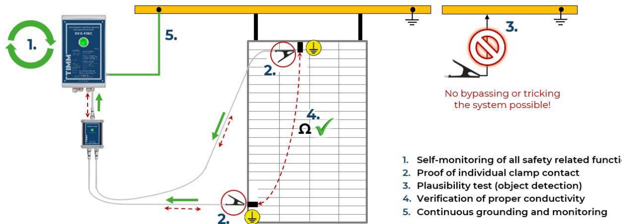
5-check measuring principle of EKX-FIBC for reliable object detection and grounding
