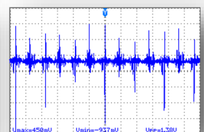
Examples of Typical EMI on Power Lines and
